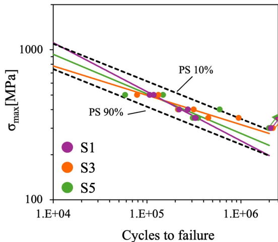
Fatigue curves-smooth specimens
