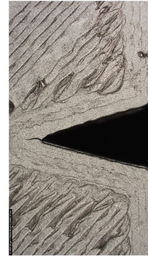
N30 ( 2\alpha=30^\circ )
