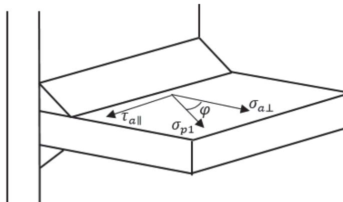
Figure 2: Illustration clarifying how angle \varphi is used to determine the maximum principal stress direction \sigma_{p1} with respect to the weld toe; Reproduced from [21].
