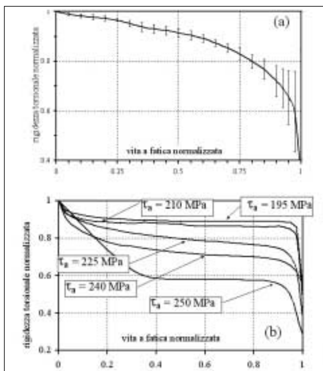
Fig. 5 - Plots of the normalised stiffness for notched (a) and plain (b) specimens.
