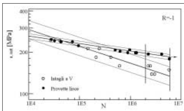
Fig. 4 - Fatigue strength data from pure torsion tests on plain and notched specimens [16].
