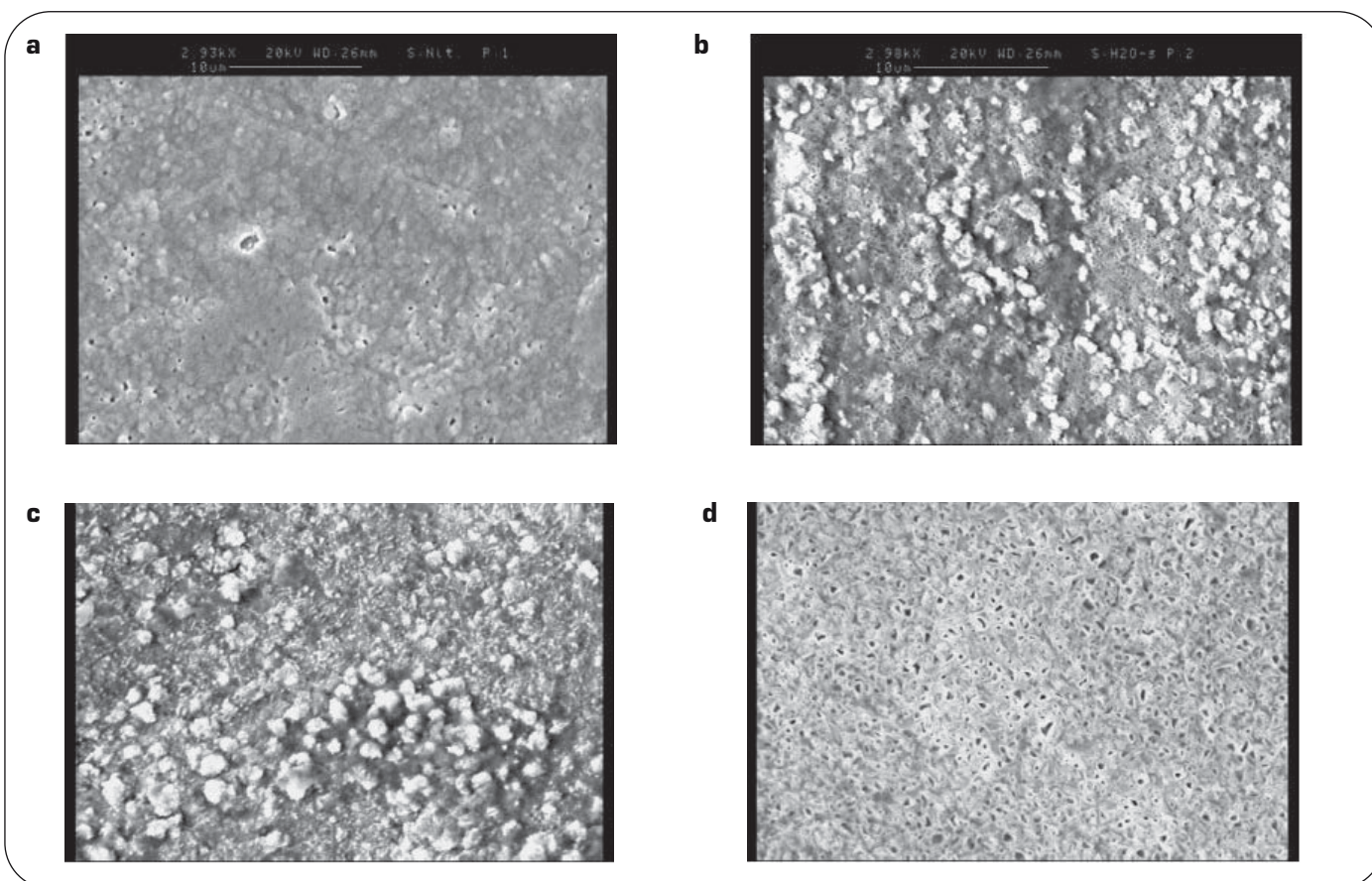
Fig. 3 Aspetto superficiale dei quattro trattamenti studiati. a) Provini nitrurati; b) Provini post-ossidati in \text{H}_2\text{O} ; c) Provini post-ossidati in \text{NO}_x ; d) Provini post-ossidati in \text{CO}_2 . SEM surface micrographs of tested samples. a) Nitrided specimen; b) Nitrided and \text{H}_2\text{O} post-ox specimen; c) Nitrided and \text{NO}_x post-ox specimen; d) Nitrided and \text{CO}_2 post-ox specimen.
