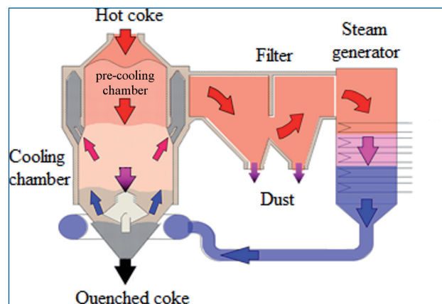
Fig. 8 - Layout of the Coke Dry Quenching System.
