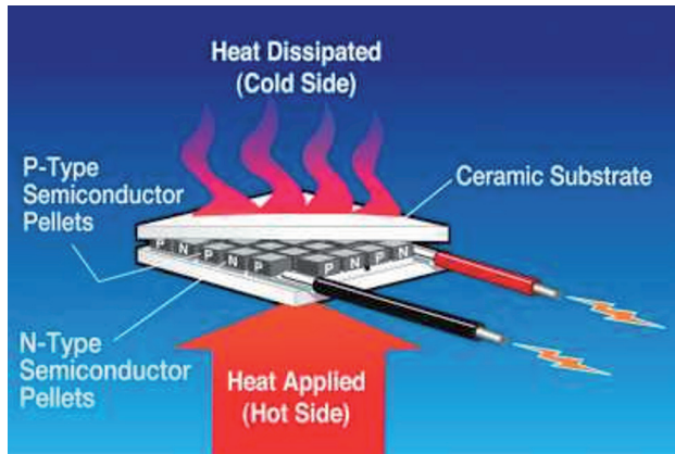
Fig. 9 - Layout of a thermoelectric module.
