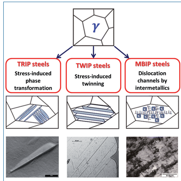
Fig. 16 - Strengthening phenomena featured in austenitic-based steels.
