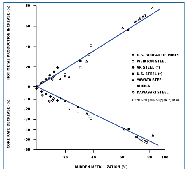
Fig. 4 - Reduction in coke consumption and increase in the production rate of the Blast Furnace as a function of DRI/HBI addition 3 .
