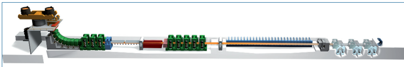
Fig. 12 - Lay-out of the Arvedi ESP process (from the continuous casting machine to coiling).
