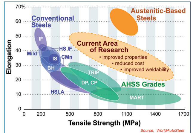
Fig. 14 - Relation between elongation (ductility) and tensile strength in low carbon steel for general applications.
