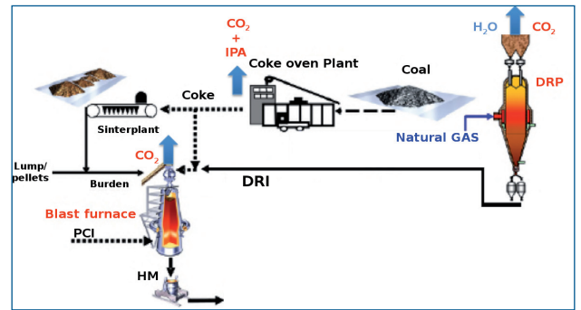
Fig. 3 - Hybrid configuration combining the pre-reduction route and the blast furnace (HM- Hot Metal pig iron /DRP Direct Reduction Process).
