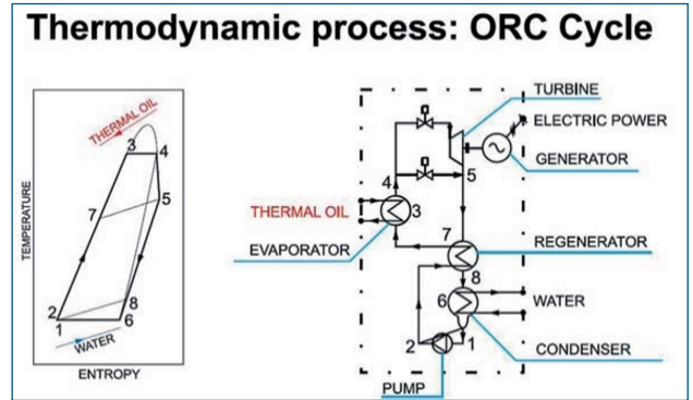
Fig. 10 - The thermodynamics of ORC.
