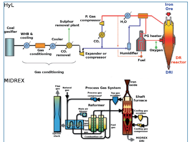
Fig. 2 - Scheme of HYL ® and MIDREX ® Processes.
