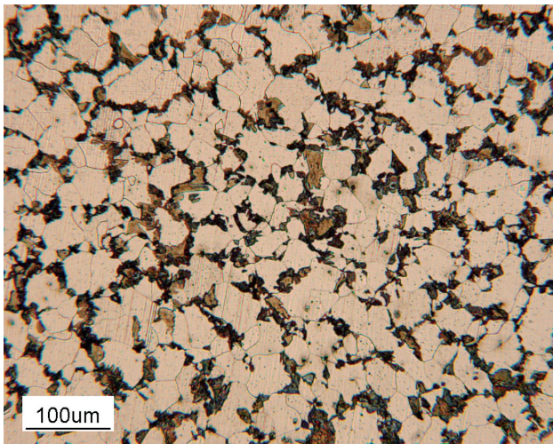
Fig. 15 - Dual Phase steel microstructure: finely dispersed hard martensitic phase (colored grains) within a soft ferritic matrix (white grains).
