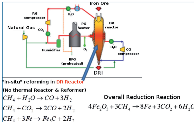
Fig. 1 - Layout of the process and the overall reduction reaction.
