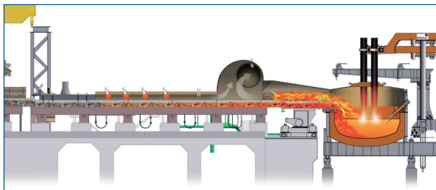
Fig. 6 - TENOVA Consteel Technology®: the outgoing fumes preheat the continuously charged steel scrap along the charging tunnel.
