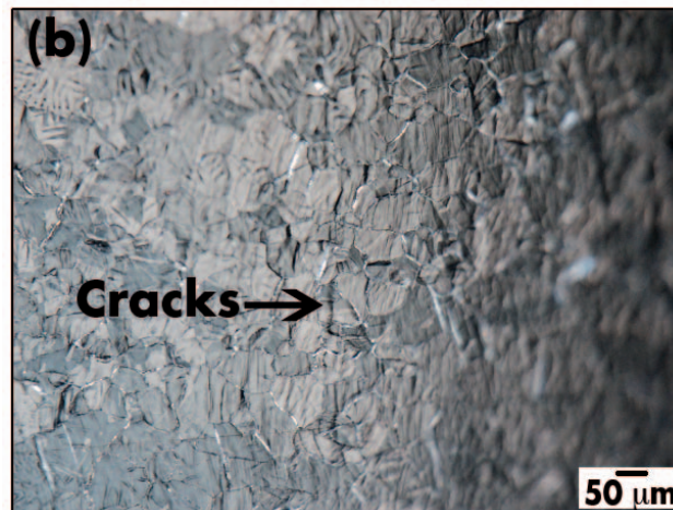
Fig 9: Stereo-micrographs of the top surface of 180° 'U' bend galvanized samples: (a) steel 1 and (b) steel 2.
