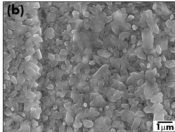
Fig 8: SEM micrographs of inhibition layer after the Zn overlay was stripped with fuming \text{HNO}_3 (a) steel 1 and (b) steel 2.
