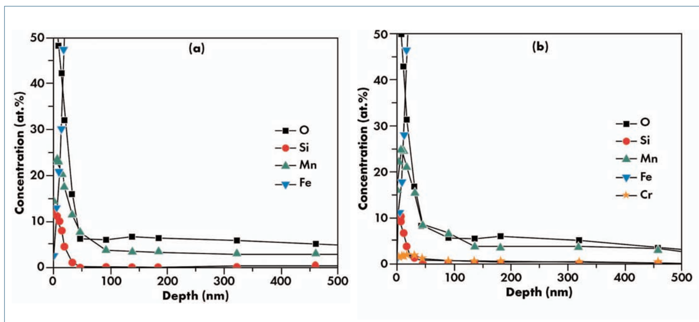
Fig 5: XPS depth profile of oxides formed on surface during annealing of (a) steel 1 and (b) steel 2.
