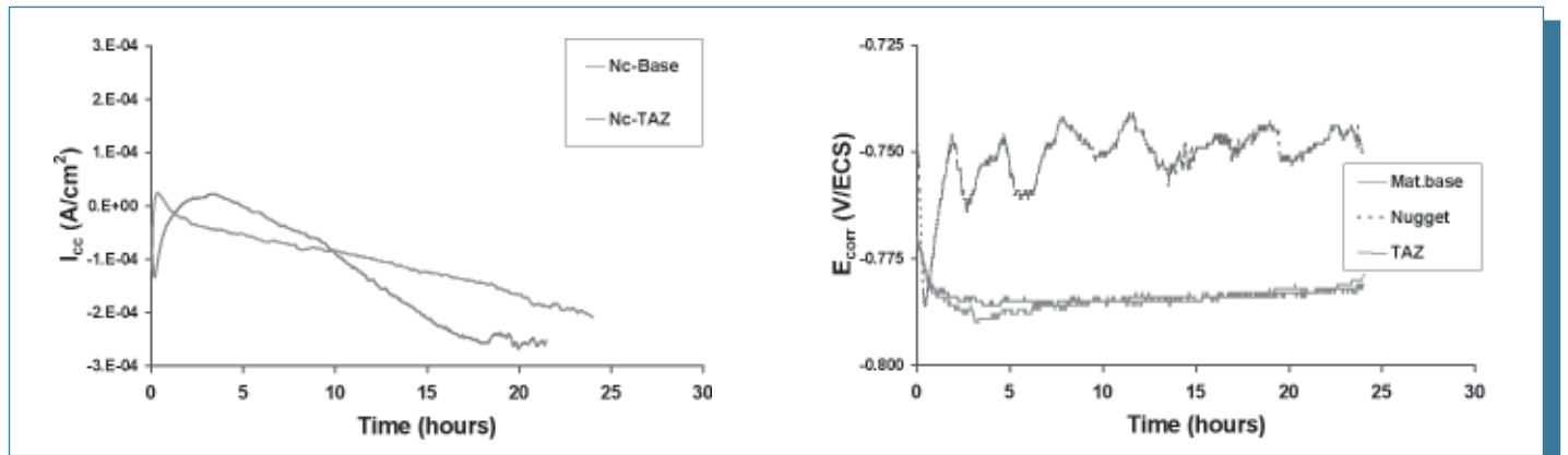
Fig. 6: Short-circuit currents and corrosion potentials of the characteristic zones of the W6A20A joint in EXCO solution
