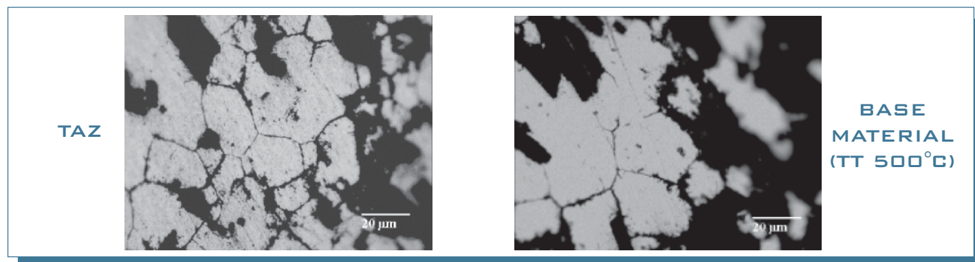
Fig. 9: Optical microscope micrographs of the TAZ and of the base material of the W6A20A joint after thermal treatment at 500°C and exposure to EXCO solution
