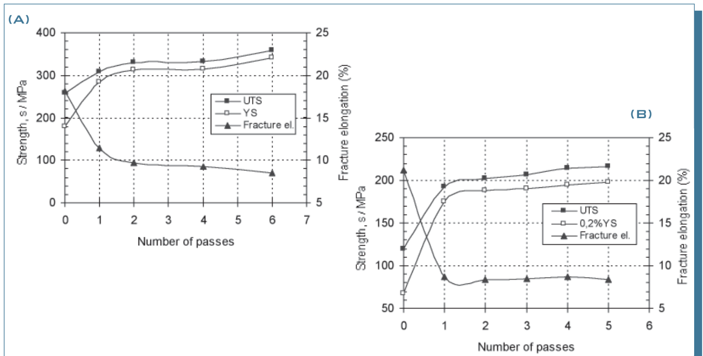
Fig. 4: Tensile properties of the 6082 alloy. (a) solution treated, ECAP processed and aged; (b) annealed and ECAP processed.
