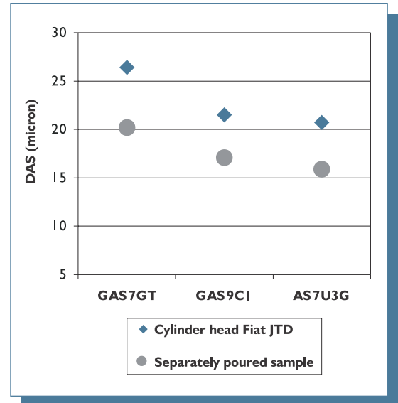
Fig. 7: DAS of different alloys, poured in separately mold and in the same cylinder head.
