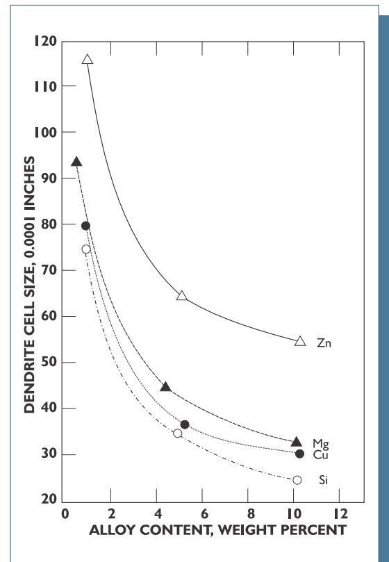
Fig. 8: Relationship between alloy content and dendrite cell size for four alloying elements in aluminium. The cooling rate for all alloys was 0,75 F/sec. By Spear and Gardner, "dendrite cell size" [1].
