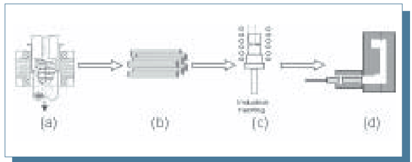
Fig. 1: Thixocasting process. Specially prepared billet is cut to length at the foundry, reheated into the semi-solid state, and finally formed into a part.
